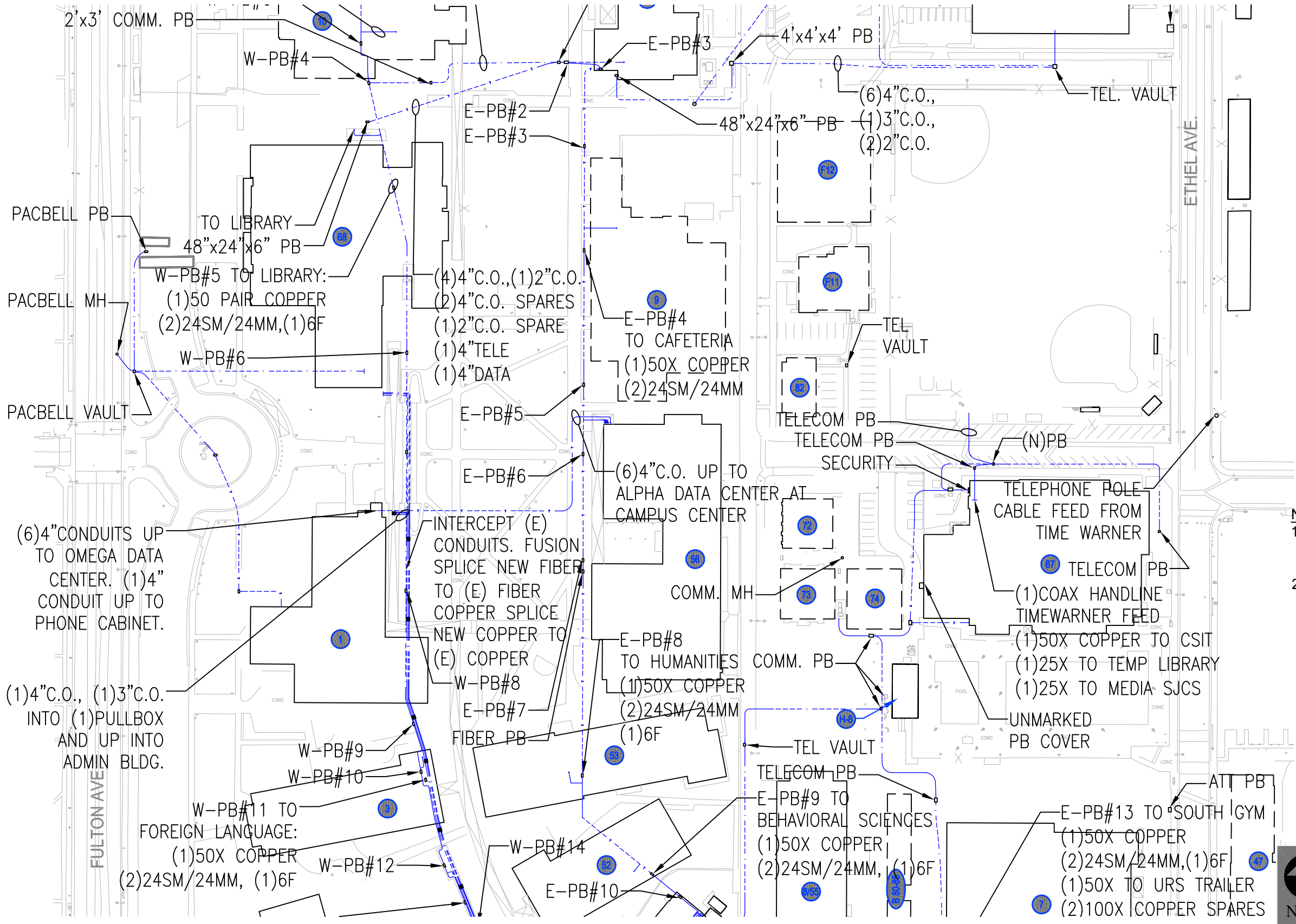
FIGURE 6b EXISTING CONDITIONS UTILITY MAP - TELECOMMUNICATIONS
