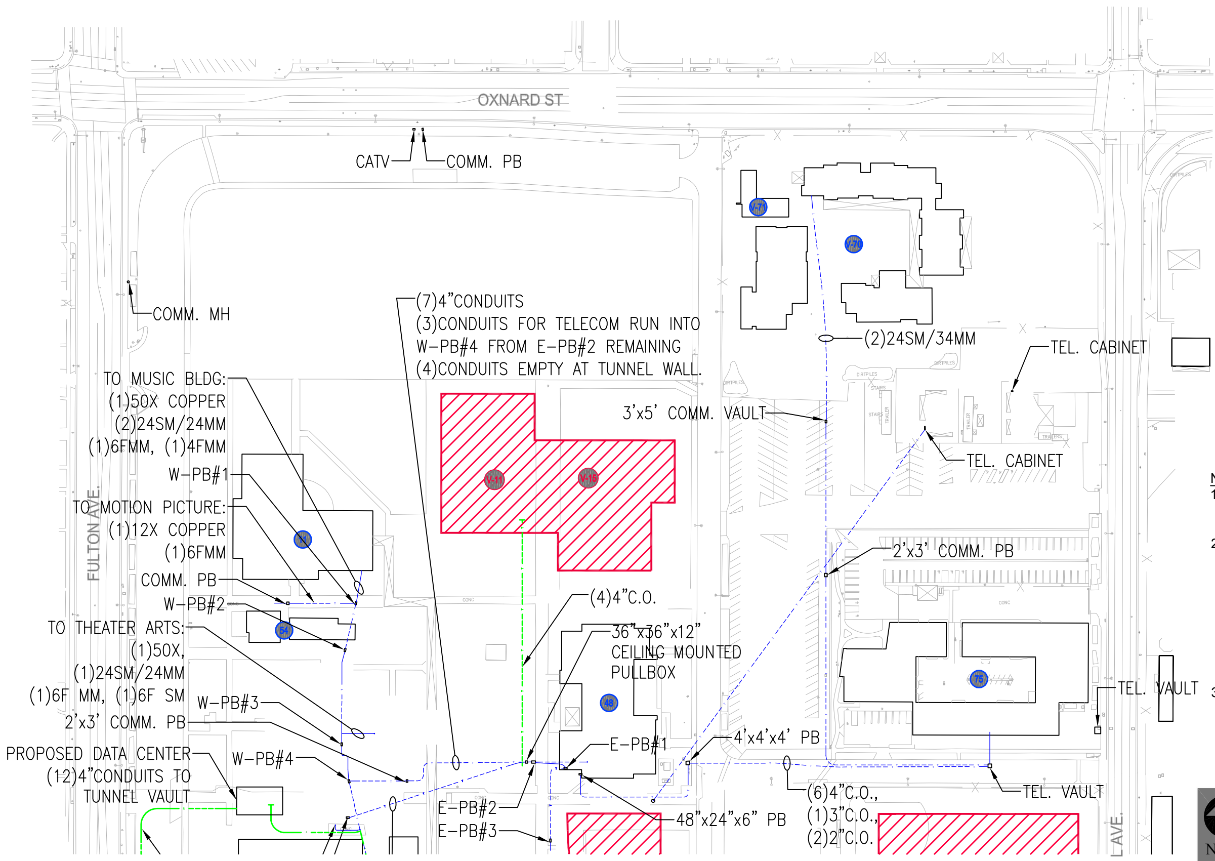
FIGURE 6e FUTURE CONDITIONS UTILITY MAP - TELECOMMUNICATIONS
