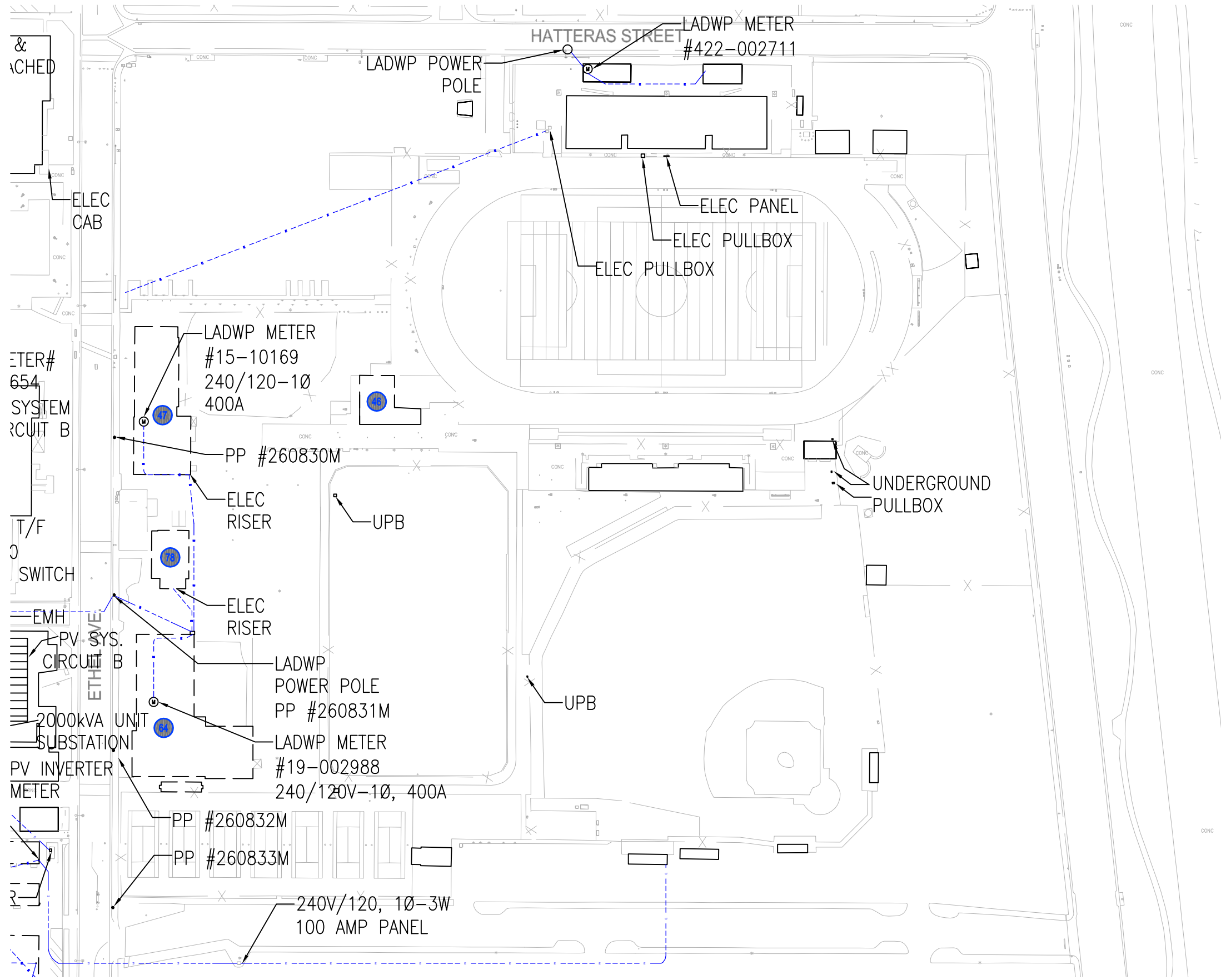
FIGURE 5d EXISTING CONDITIONS UTILITY MAP - ELECTRICAL
