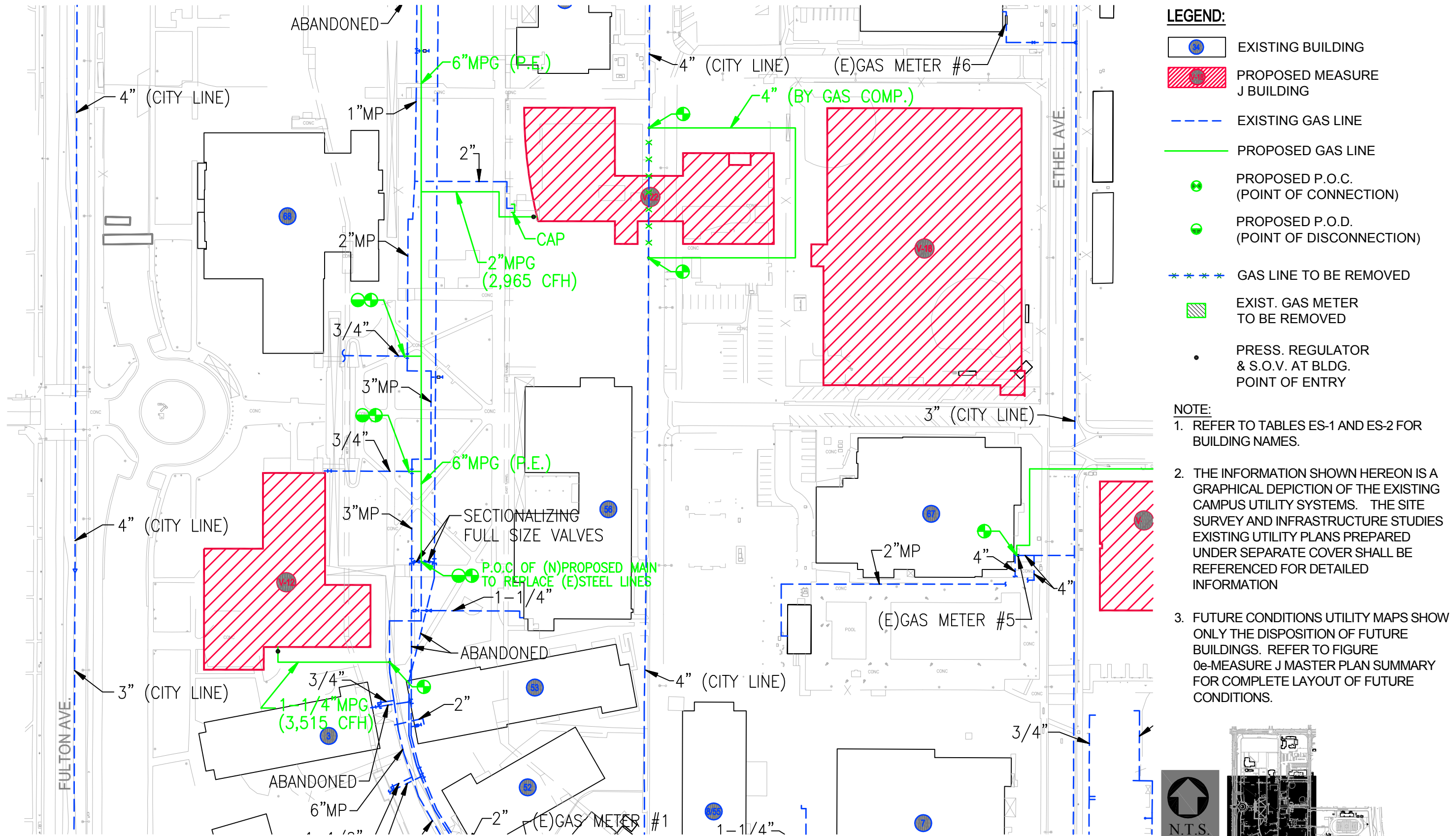
FIGURE 7f FUTURE CONDITIONS UTILITY MAP - NATURAL GAS
