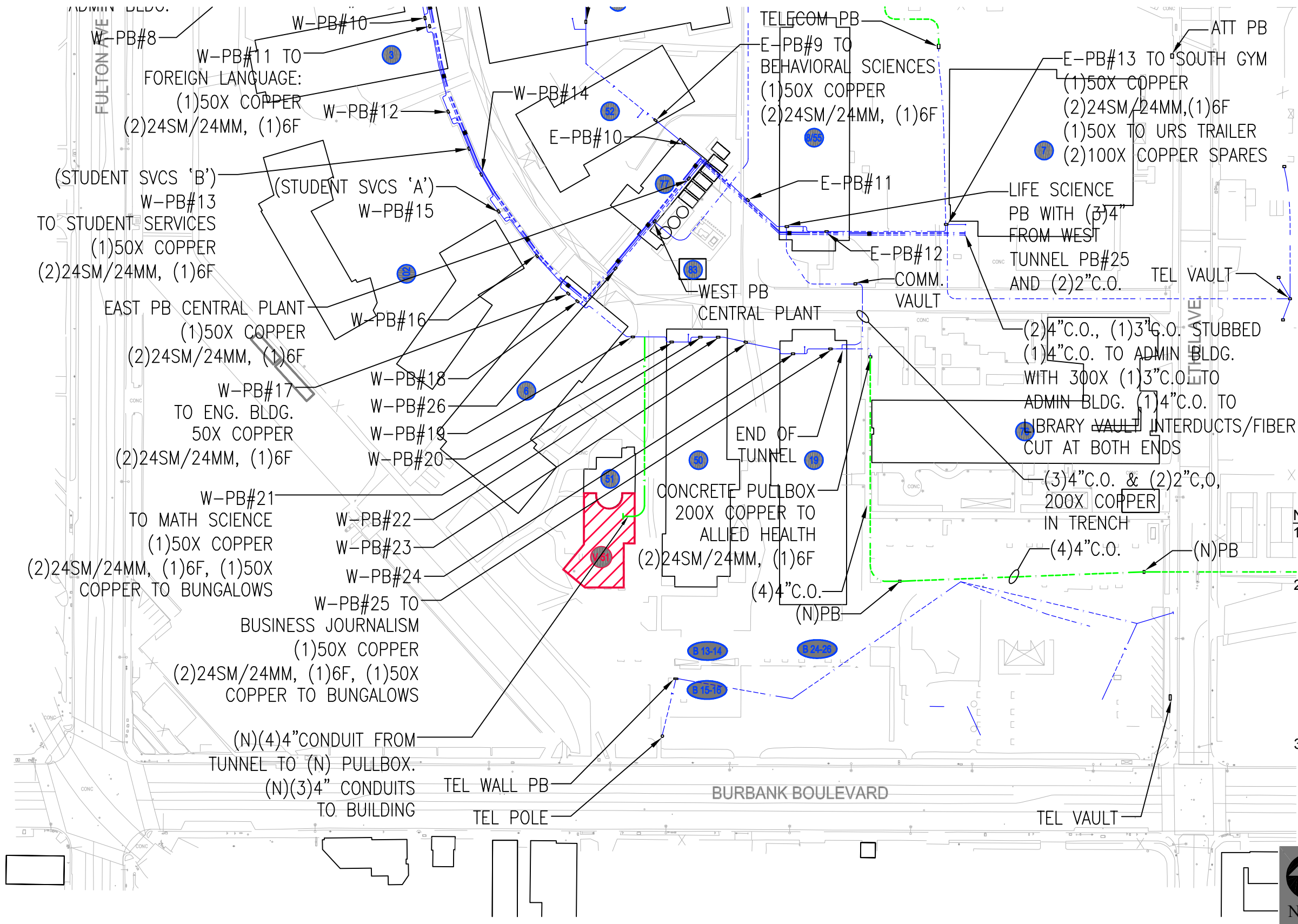
FIGURE 6g FUTURE CONDITIONS UTILITY MAP - TELECOMMUNICATIONS
