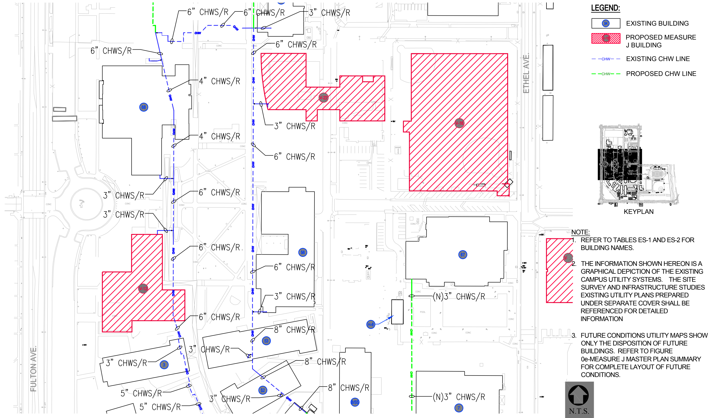
FIGURE 8f FUTURE CONDITIONS UTILITY MAP - CHILLED WATER
