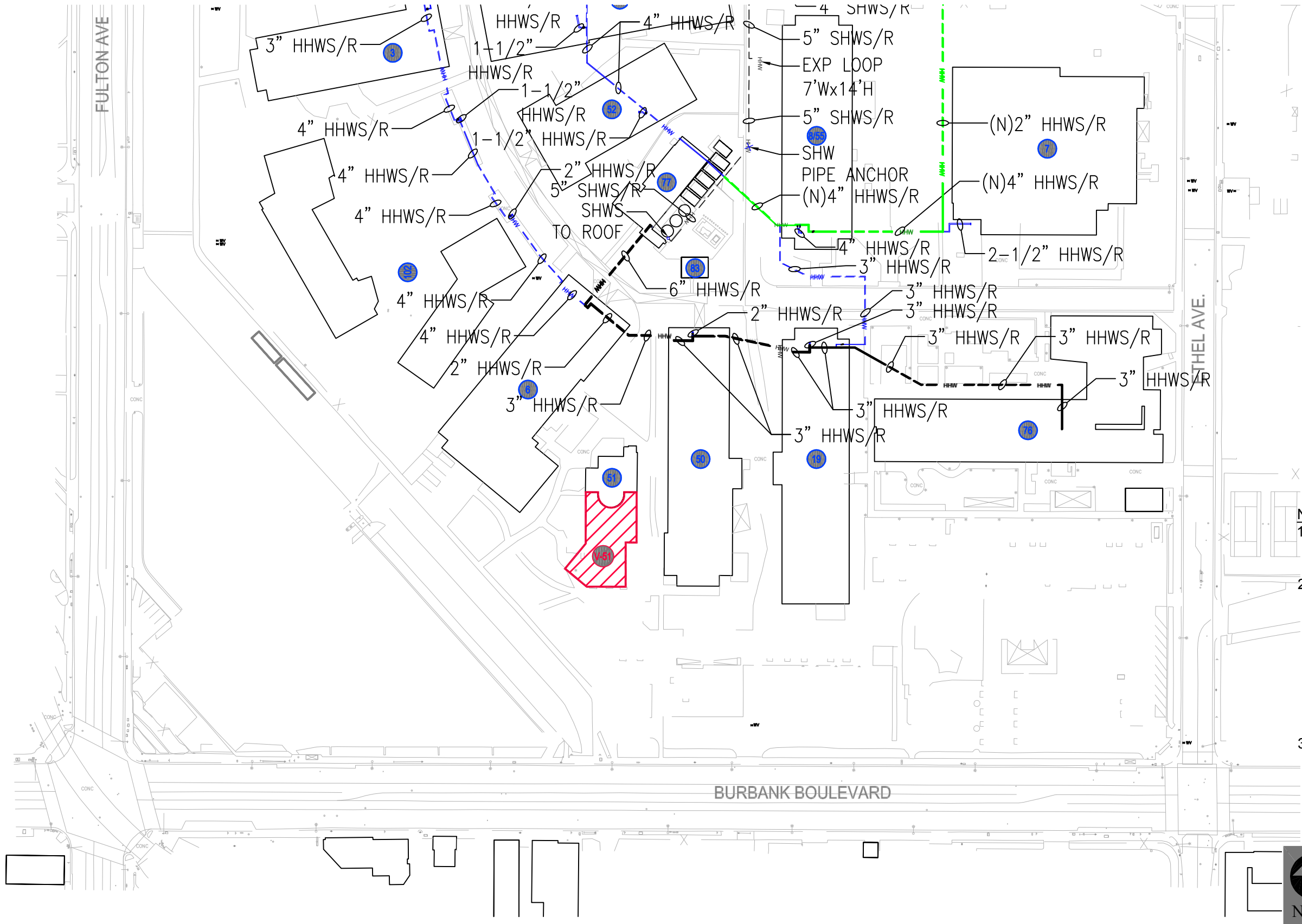
FIGURE 9g FUTURE CONDITIONS UTILITY MAP - HOT WATER
