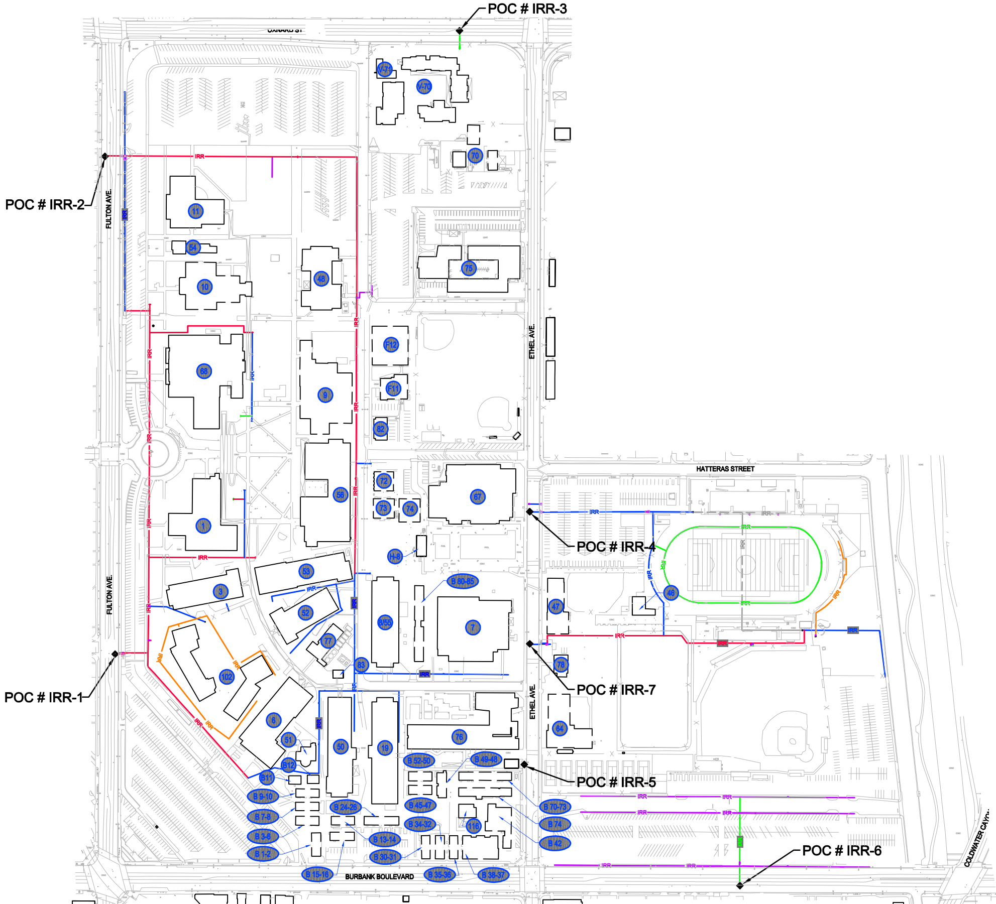
FIGURE 4a EXISTING UTILITY MAP - IRRIGATION WATER DISTRIBUTION
