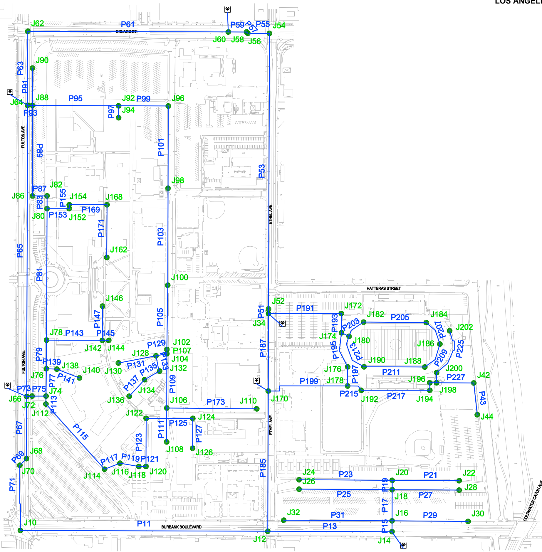
FIGURE 4c EXISTING IRRIGATION WATER DISTRIBUTION - PIPE AND NODE MAP
