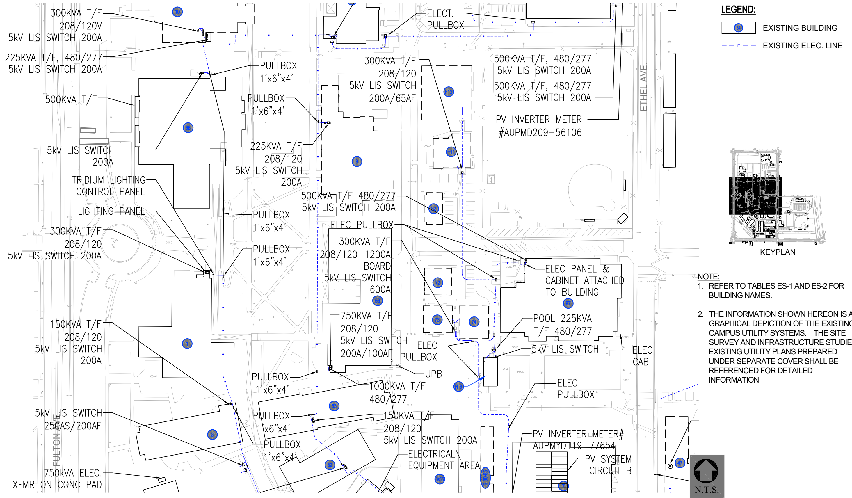
FIGURE 5b EXISTING CONDITIONS UTILITY MAP - ELECTRICAL
