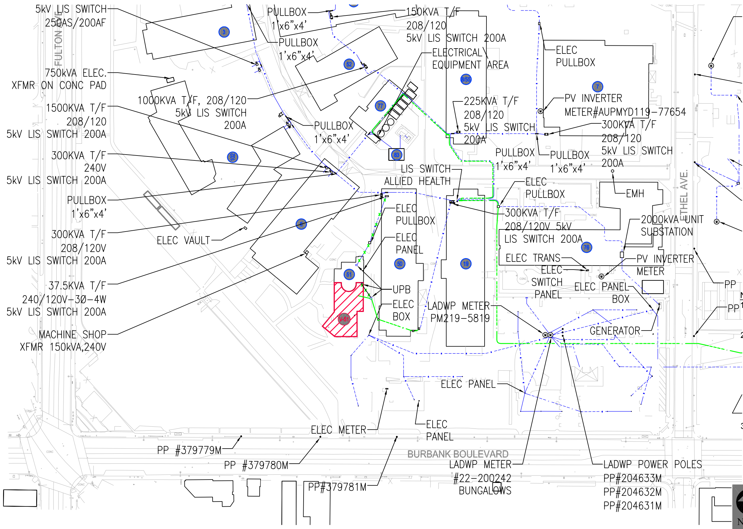
FIGURE 5h FUTURE CONDITIONS UTILITY MAP - ELECTRICAL
