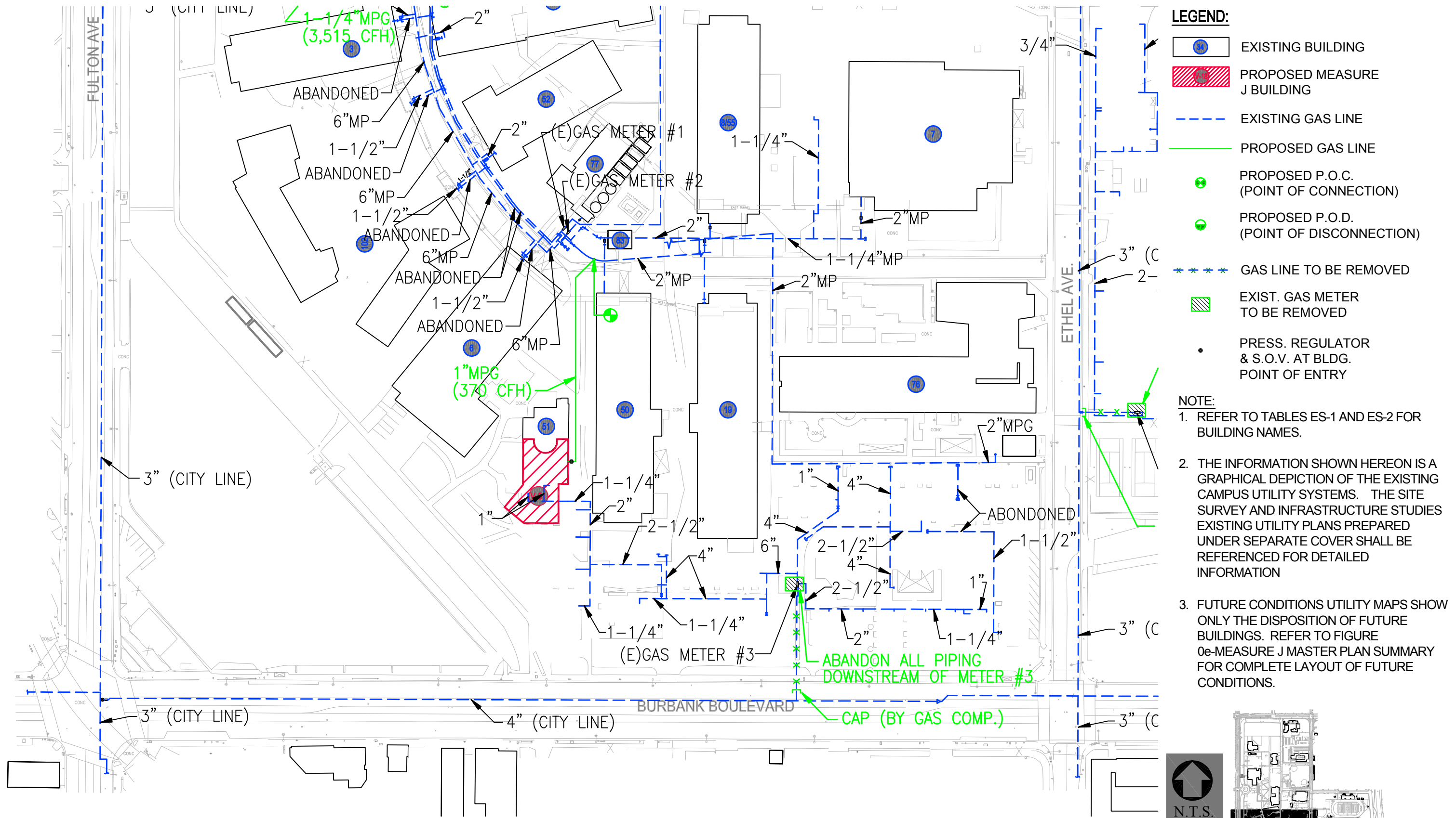
FIGURE 7g FUTURE CONDITIONS UTILITY MAP - NATURAL GAS
