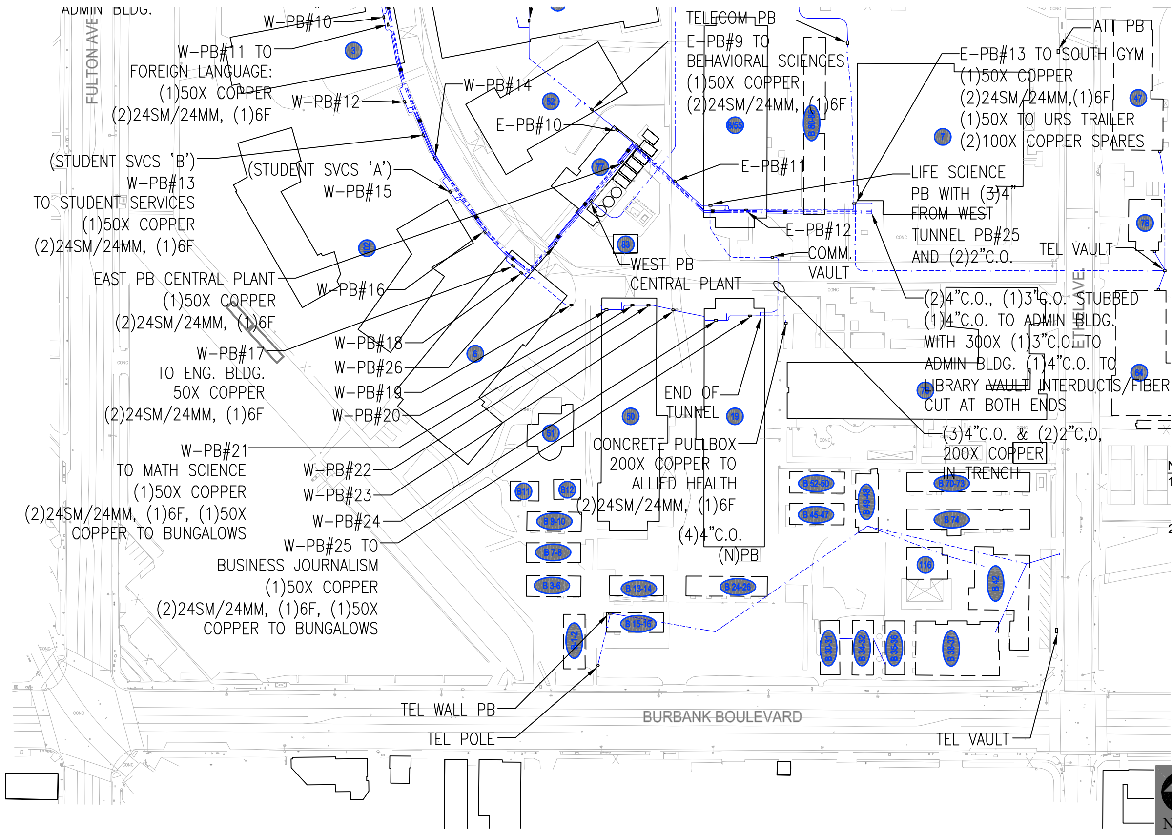
FIGURE 6c EXISTING CONDITIONS UTILITY MAP - TELECOMMUNICATIONS
