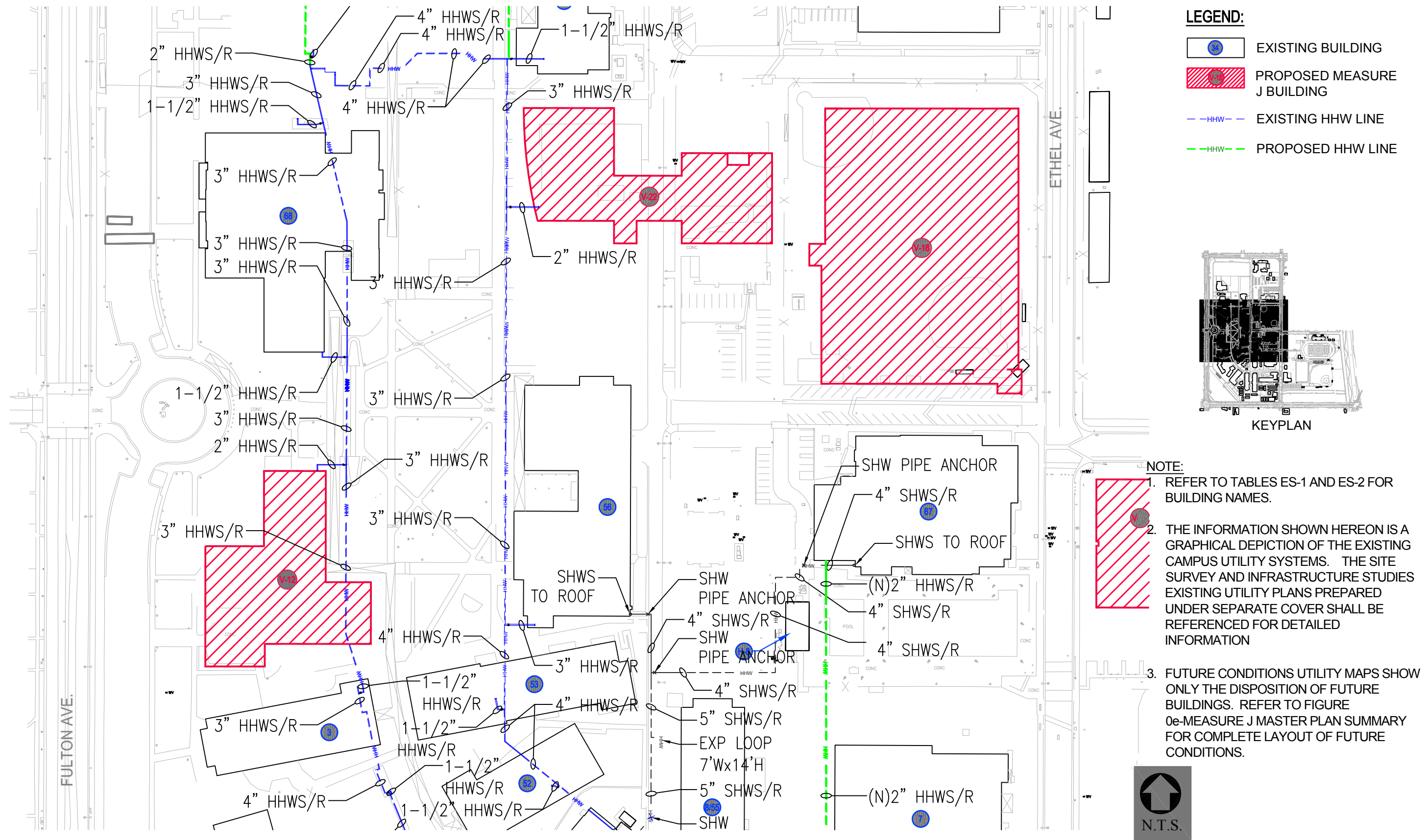
FIGURE 9f FUTURE CONDITIONS UTILITY MAP - HOT WATER
