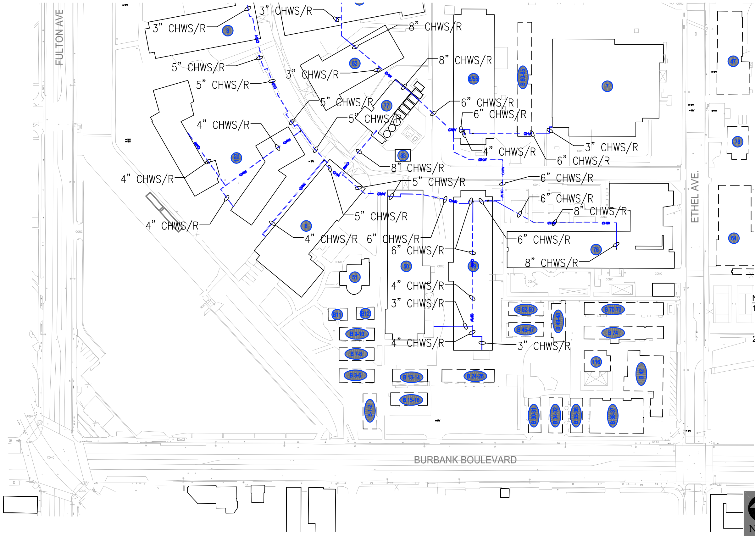
FIGURE 8c EXISTING CONDITIONS UTILITY MAP - CHILLED WATER
